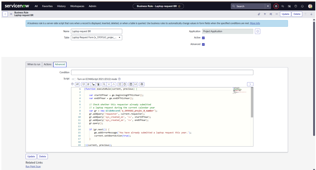
Figure 12: Business Rule for Duplicate Request Validation
