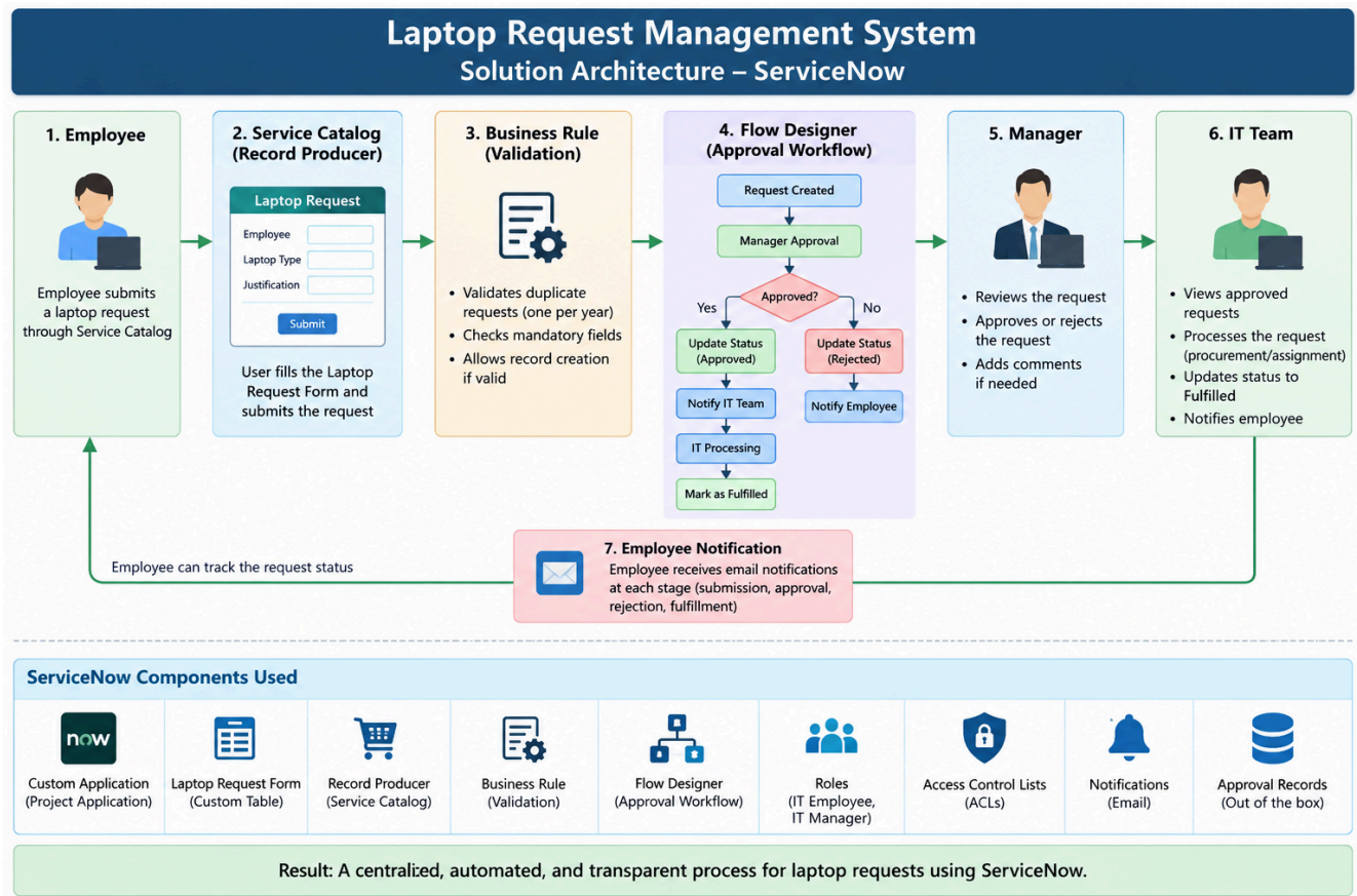
Figure 1: Solution Architecture Diagram – Laptop Request Management System
