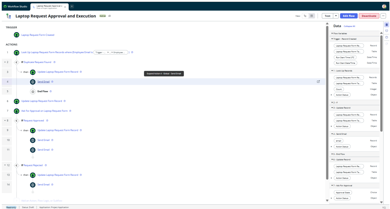
Figure 14: Laptop Request Approval and Execution Flow
